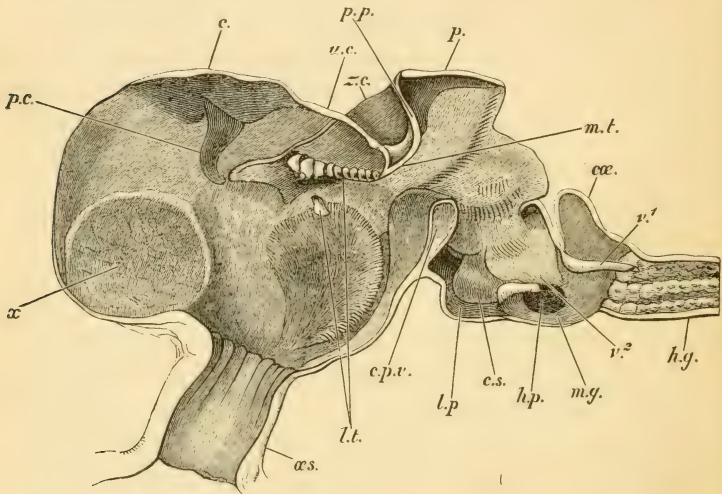
FIG. 10.— Astacus fluviatilis .—Longitudinal section of the stomach ( \times 4 ), c , cardiac ossicle; ca , caecum; c.p.v. , cardio-pyloric valve; cs , cushion-shaped surface; hg , hind-gut; hp , aperture of right bile duct; lp , lateral pouch; lt , lateral teeth; mg , mid-gut; mt , median tooth; as , oesophagus; p , pyloric ossicle; pc , ptero-cardiac ossicles; pp , prepyloric ossicle; uc , urocardiac process; v 1 , median pyloric valve; v 2 , lateral pyloric valve; x , position of gastrolith; zc , zygocardiac ossicle.
